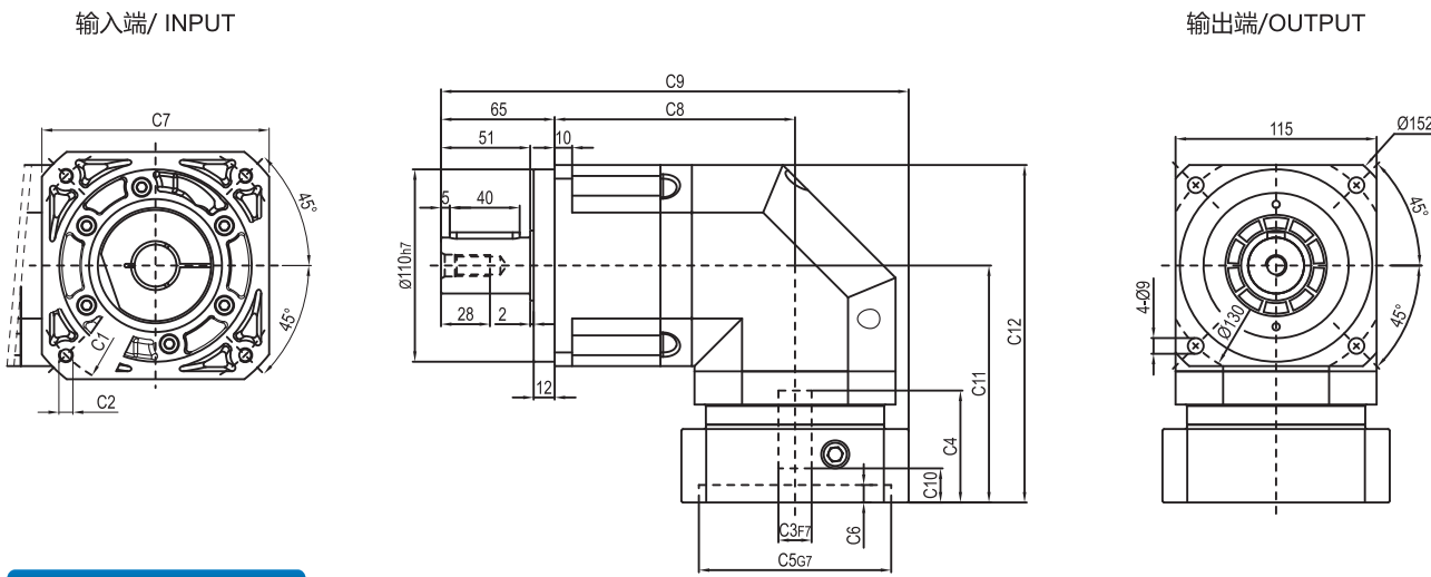
FABR-115D(M1)-L2
