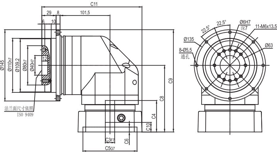
输出端/OUTPUT
