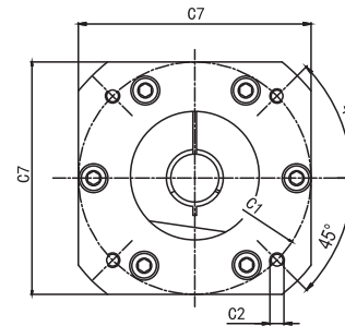
FE-235D-L2
