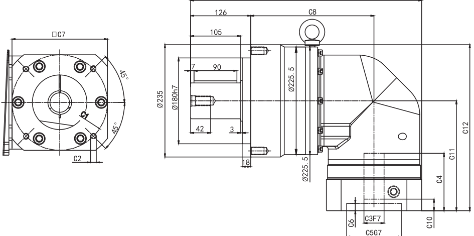
FER-235D-L2
