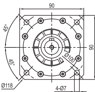
输出端/OUTPUT
