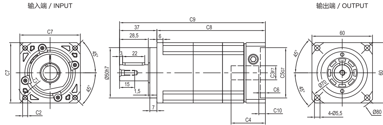
FAB-060D(M1)-L2
