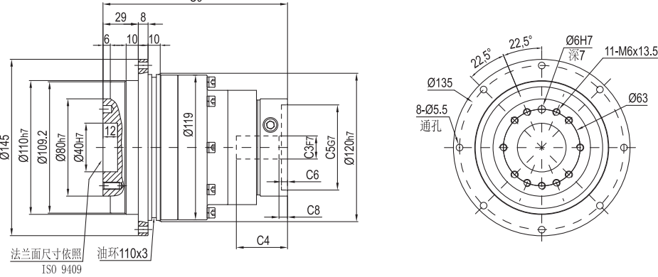
输出端/OUTPUT
