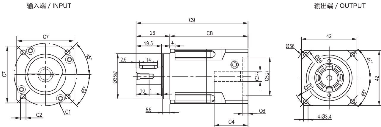
FAB-042D-L2
