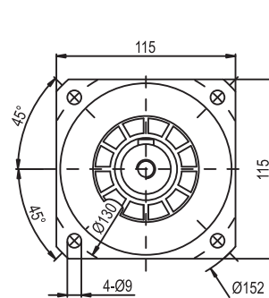
输出端/OUTPUT
